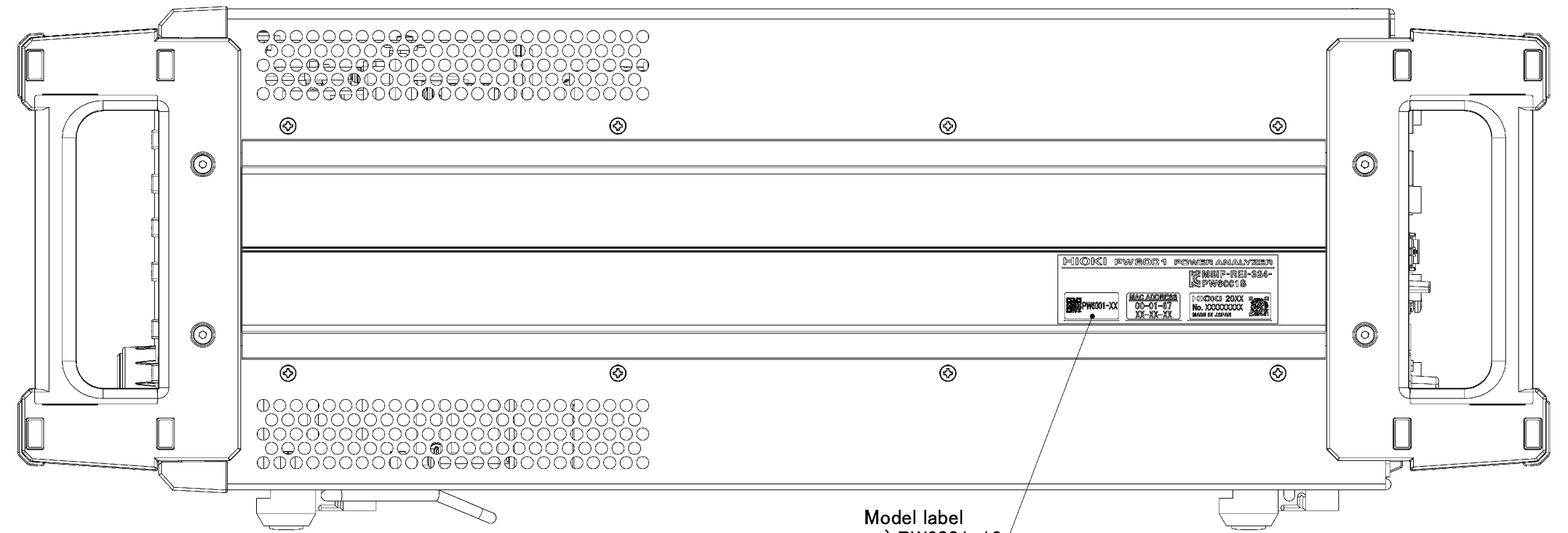
Model label ex) PW6001-16 Side view
